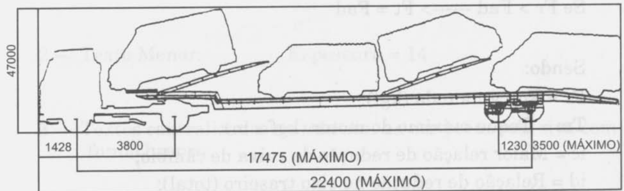
Semi-Reboque Transporte Vans
